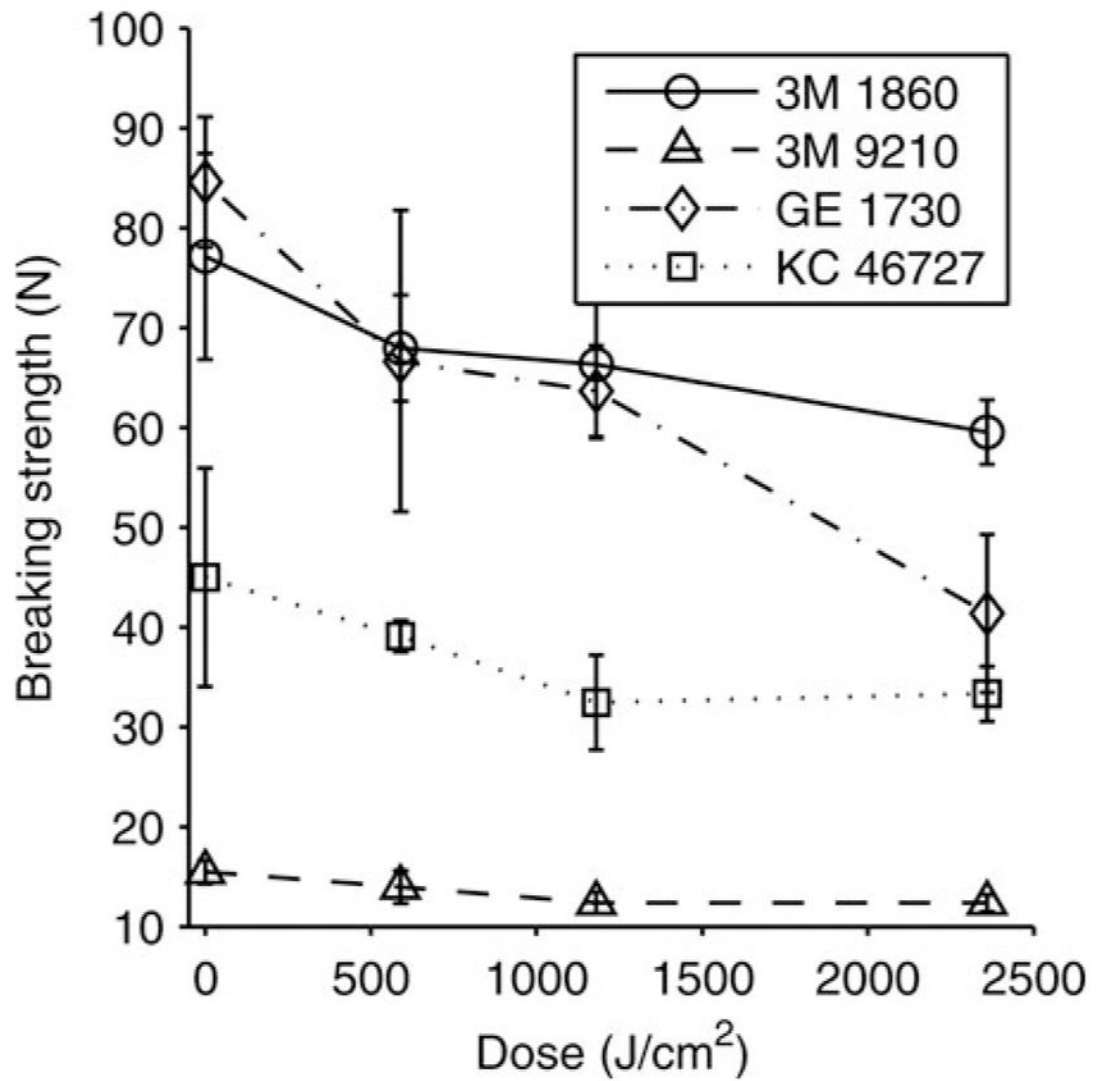
FIGURE 4. Breaking strength vs. UVGI dose for respirator straps. Each data point shows the mean breaking strength for the respirator straps exposed to the dose of UVGI. Eight straps were tested at 4 different doses, with a matched control tested for each exposed strap (32 controls total). Error bars show the standard deviation.
